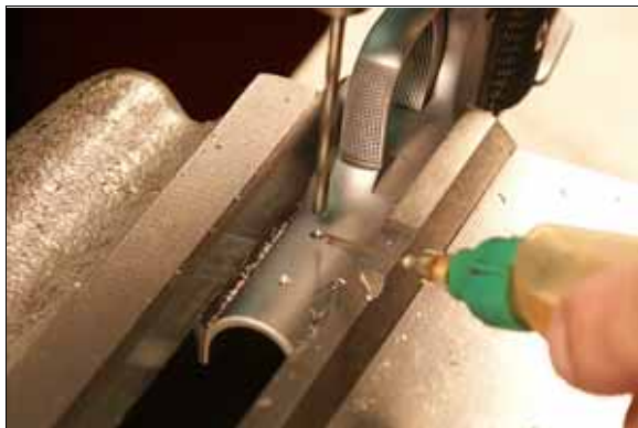
Step 7: Drill Both Holes With A #43 Drill. Lubricate While Drilling.
