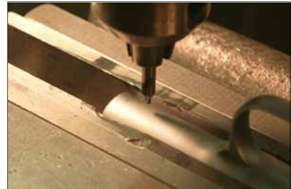
Step 5: Drill Starter Hole .565" From End Of Dust Cover. Lubricate While Drilling.
